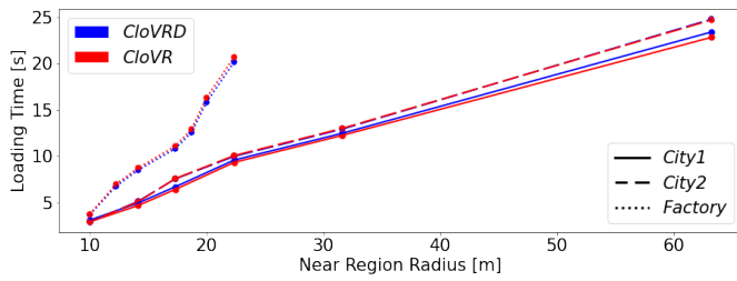
Fig. 7: Progressive loading times as a function of the growing near region radius, for the two near-far partitioning methods and the three VE locations, averaged over all Experiment 1 participants.
