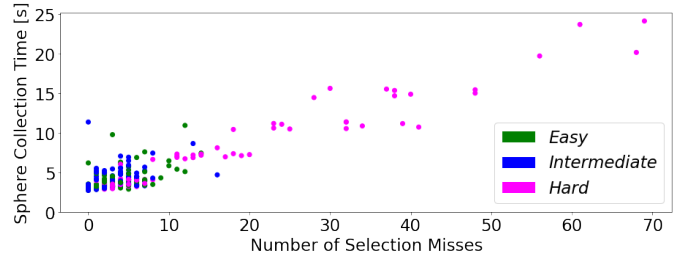
Fig. 11: The time needed to collect a sphere as a function of the number of selection misses, and of the sphere type.
