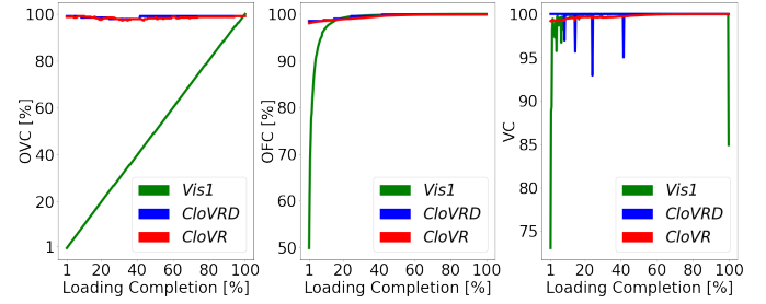
Fig. 4: Analytical comparison of loading approaches for the City VE in terms of object visualization completion (left), object footprint completion (middle), and visual continuity (right).
